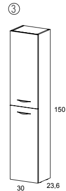
Columna Column MAXIMUM
